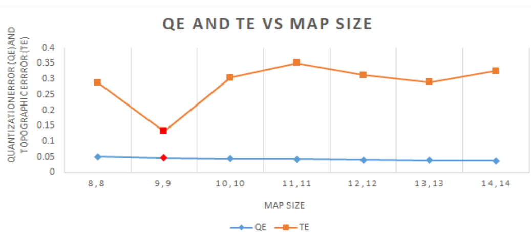
Fig. 6 Plot of Quantization Error and Topographic Error with a fixed learning rate of 0.5 and fixed number of iterations of 8000
