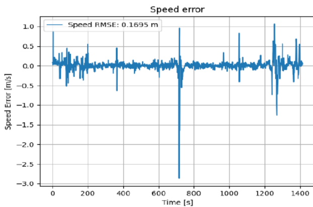
Fig 6: Speed error calculated based on ground truth
